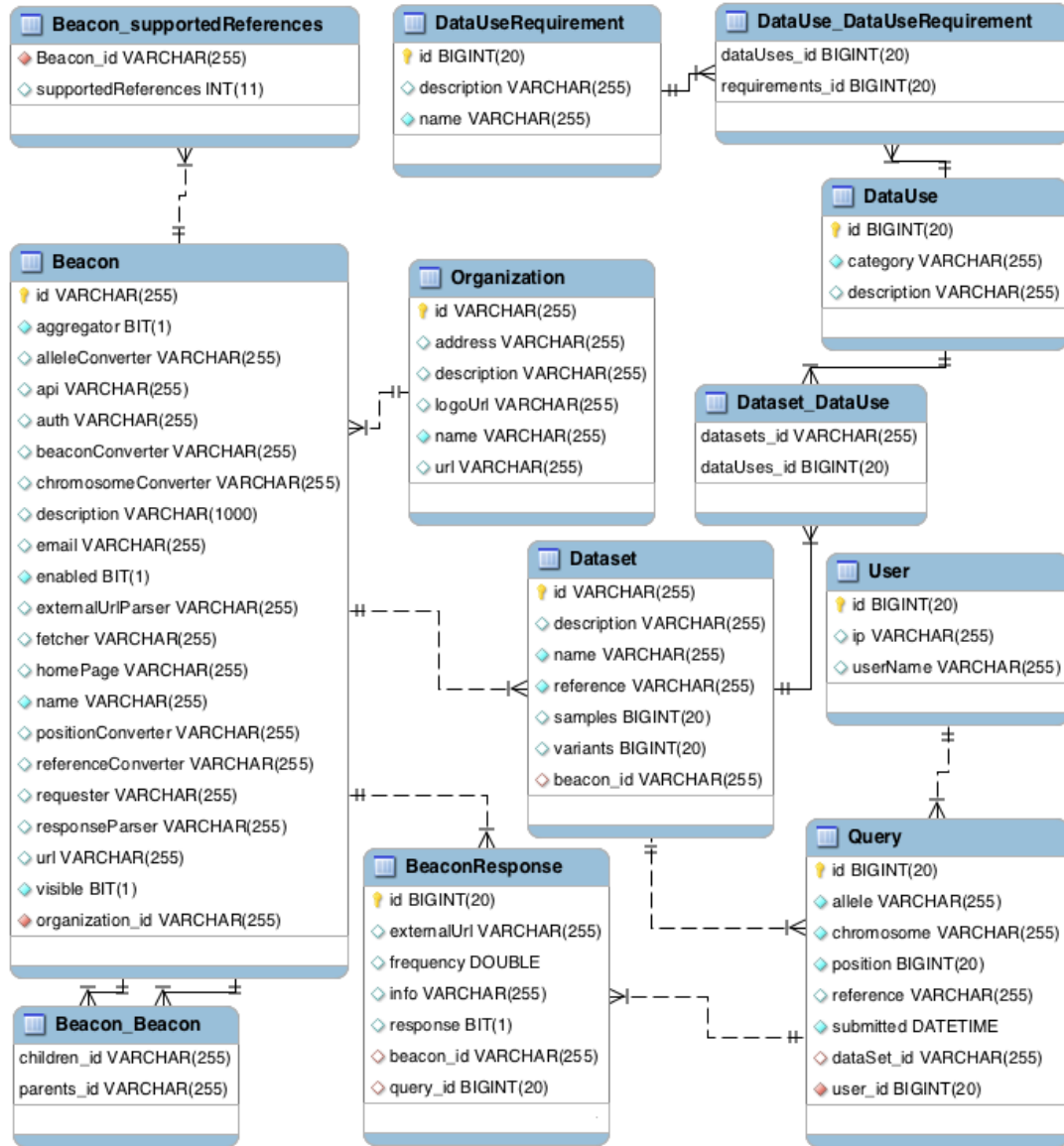
Figure 3.3: Entity-relationship diagram showing the data model of the Beacon Network.
